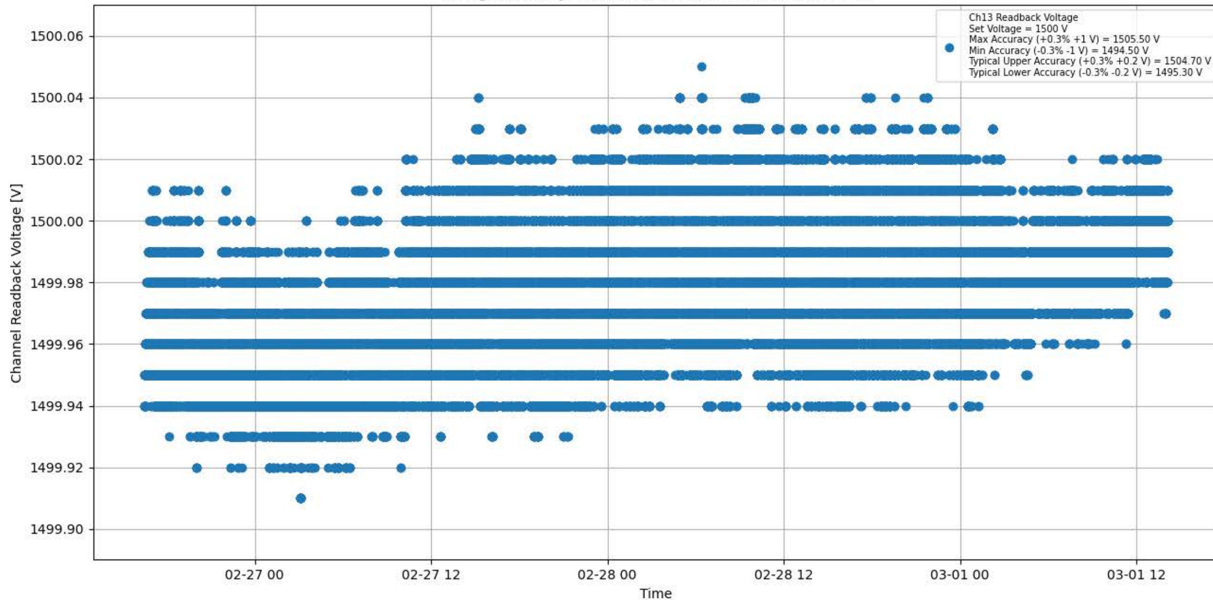
Voltage Stability 1500 V for Module #083 Channel #13
