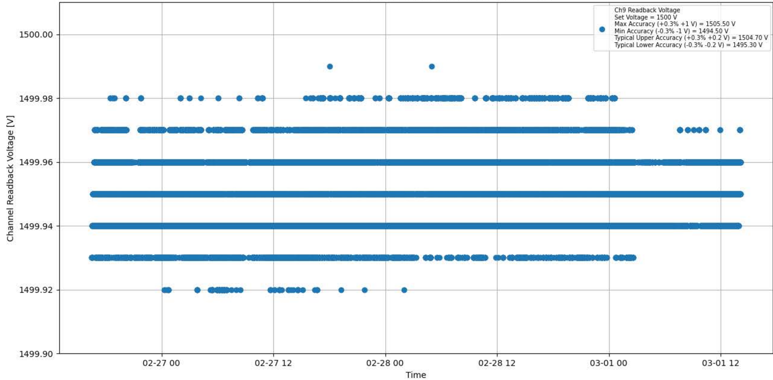
Voltage Stability 1500 V for Module #083 Channel #9
