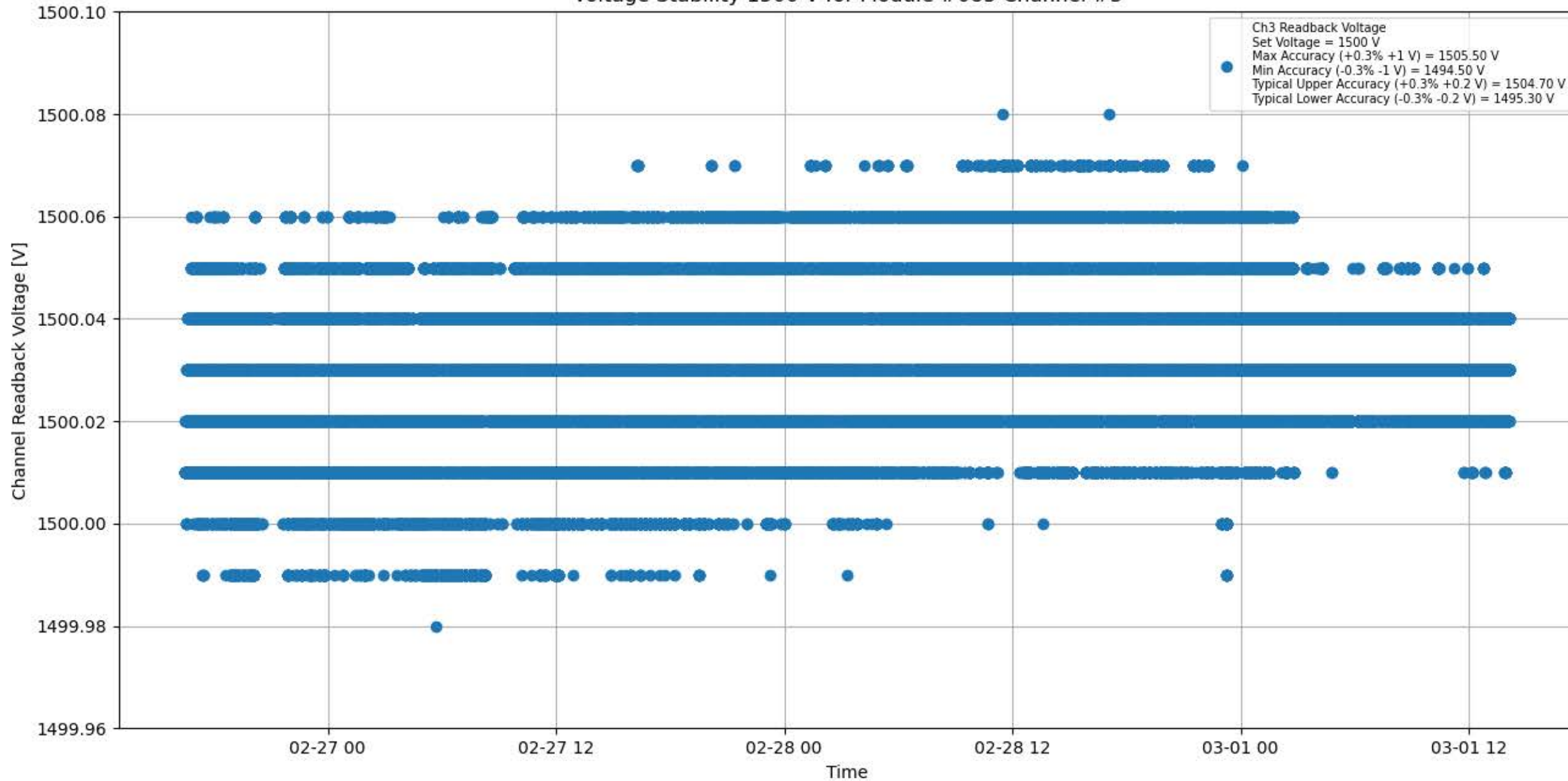
Voltage Stability 1500 V for Module #083 Channel #3
