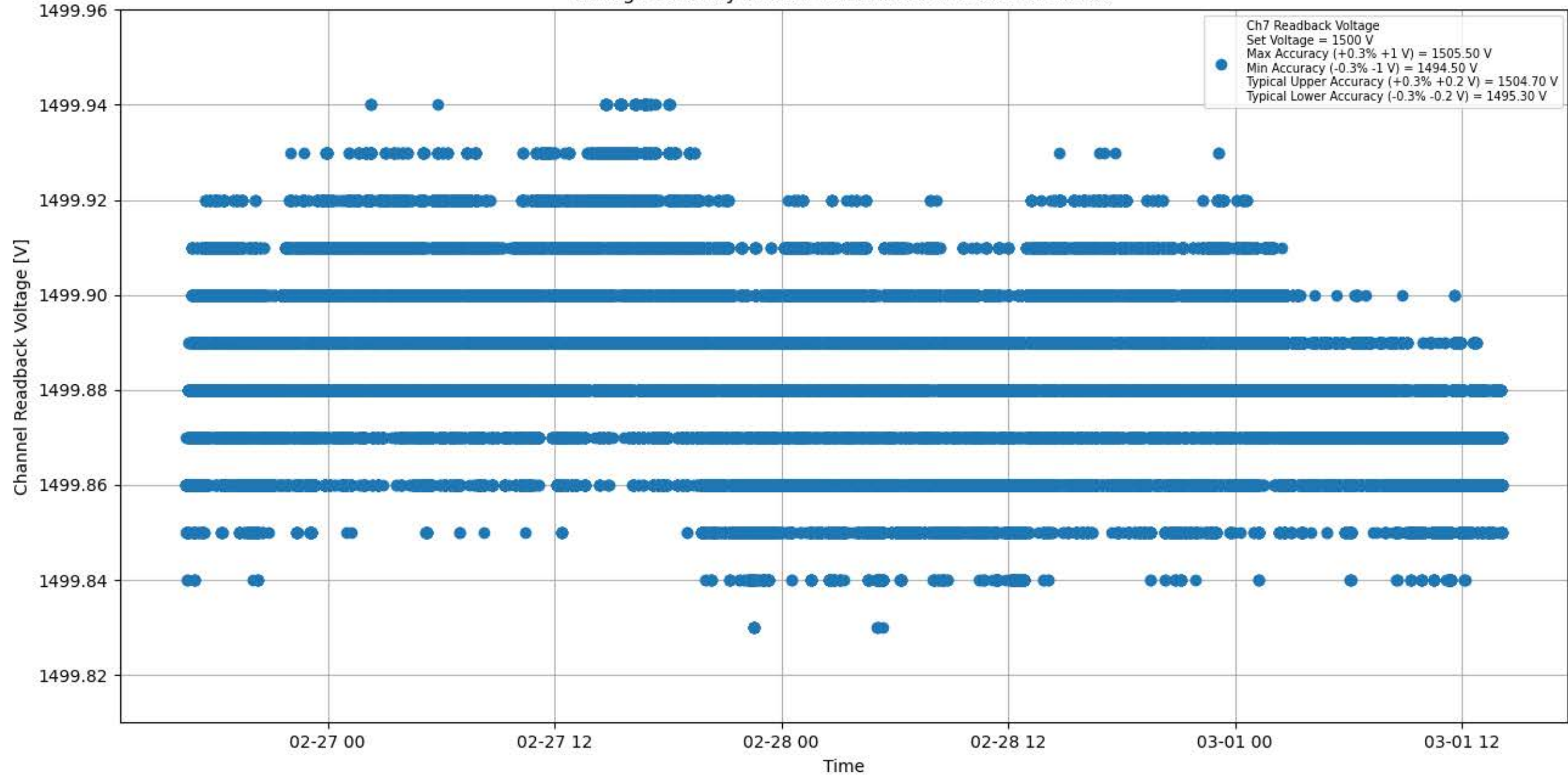
Voltage Stability 1500 V for Module #083 Channel #7
