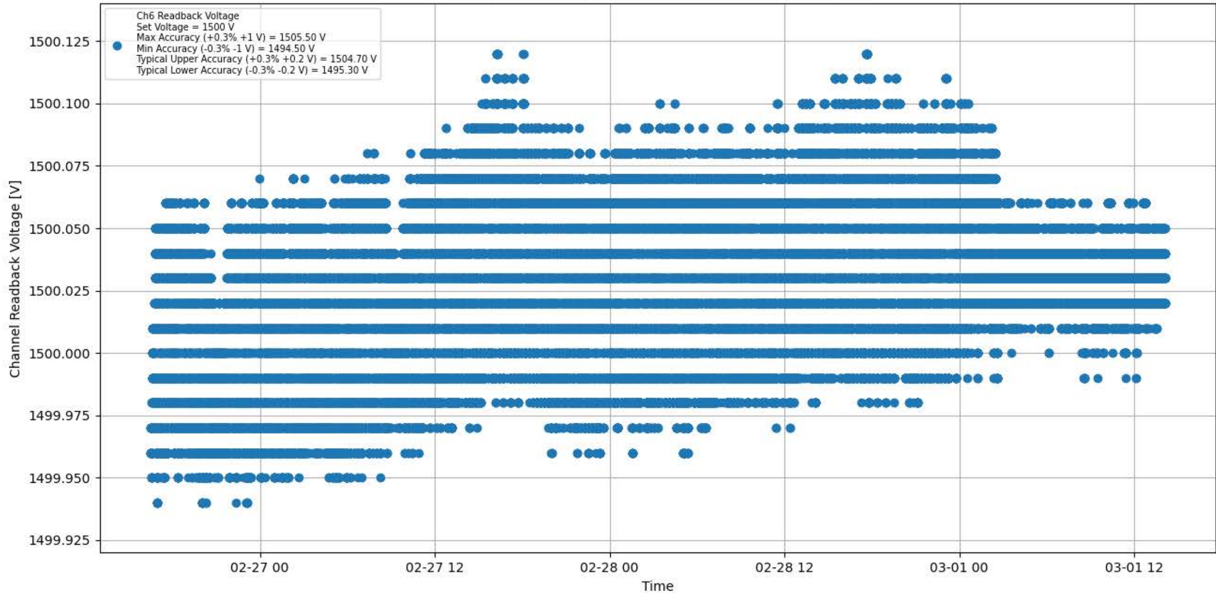
Voltage Stability 1500 V for Module #083 Channel #6
