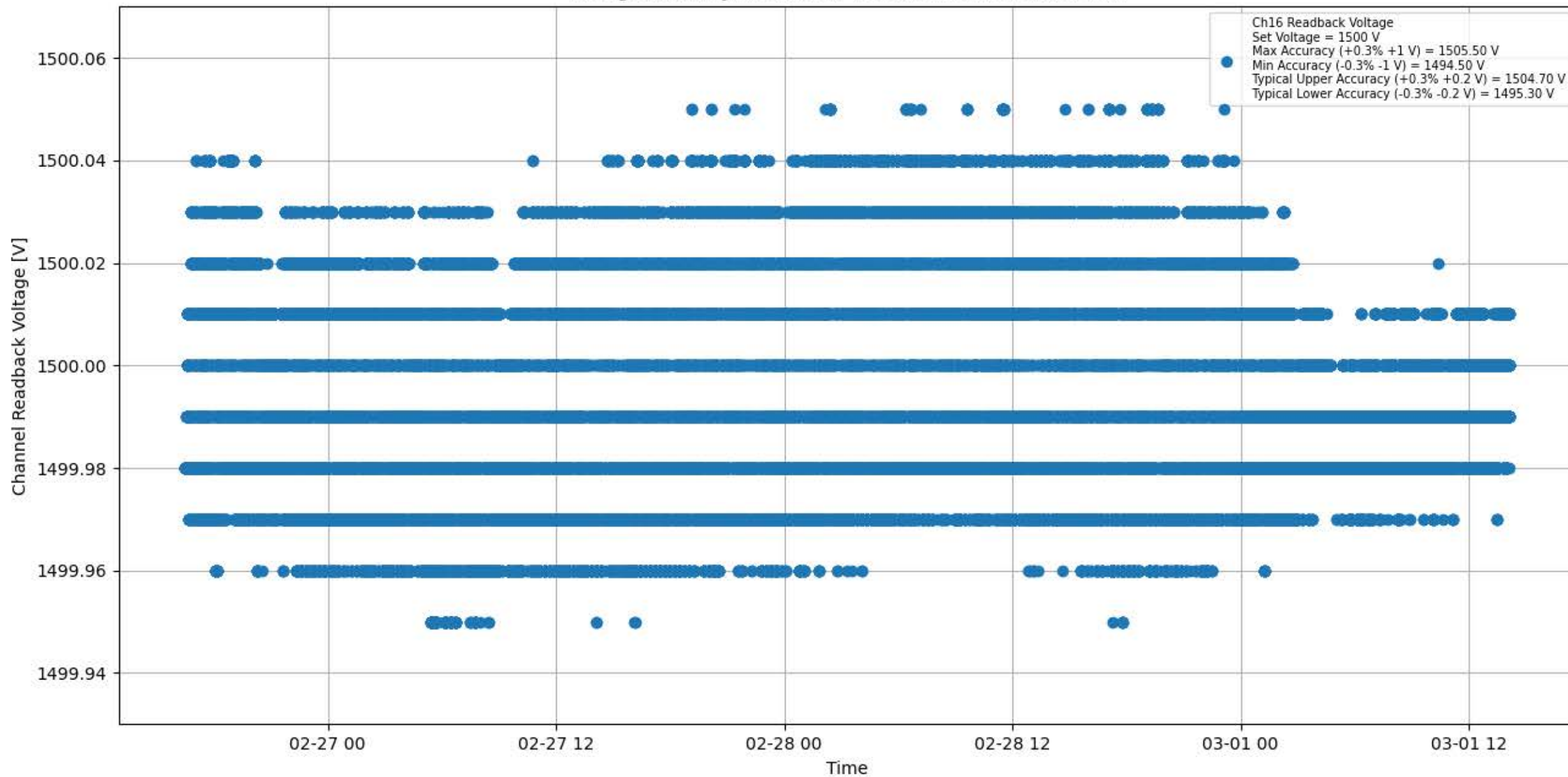
Voltage Stability 1500 V for Module #083 Channel #16
