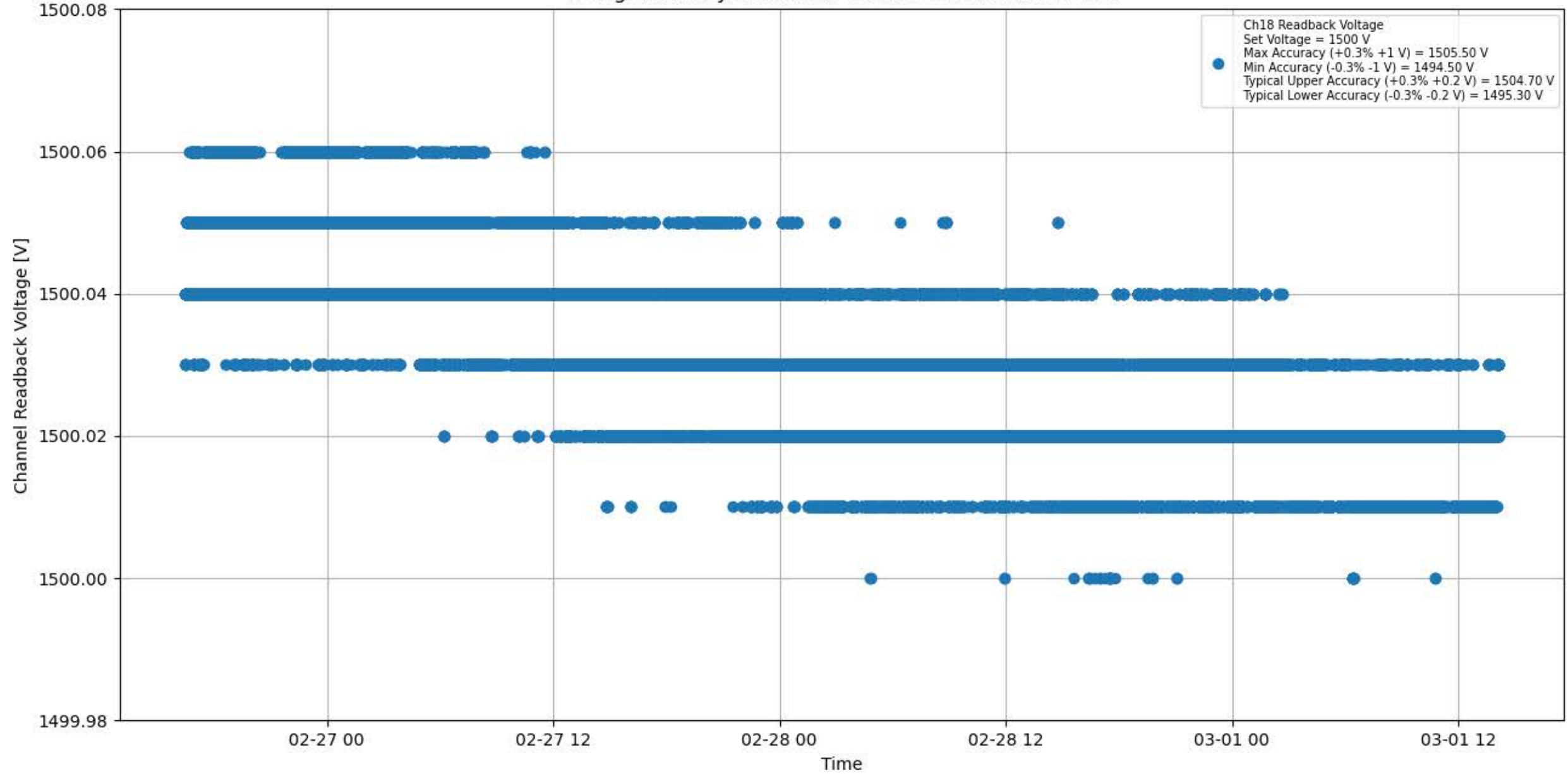
Voltage Stability 1500 V for Module #083 Channel #18
