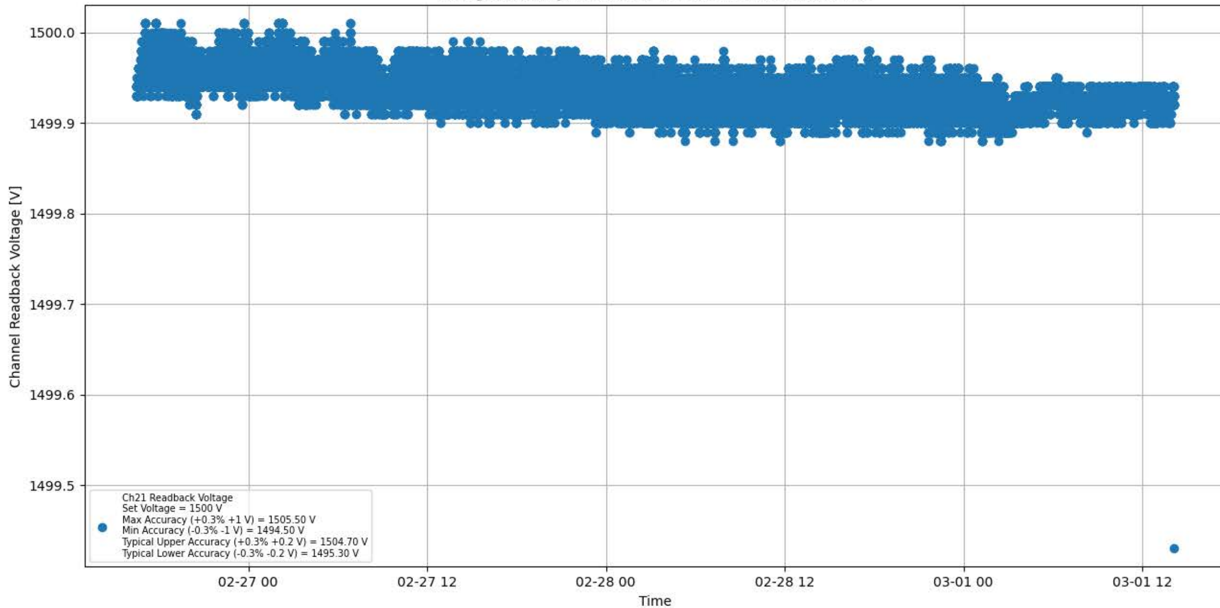
Voltage Stability 1500 V for Module #083 Channel #21
