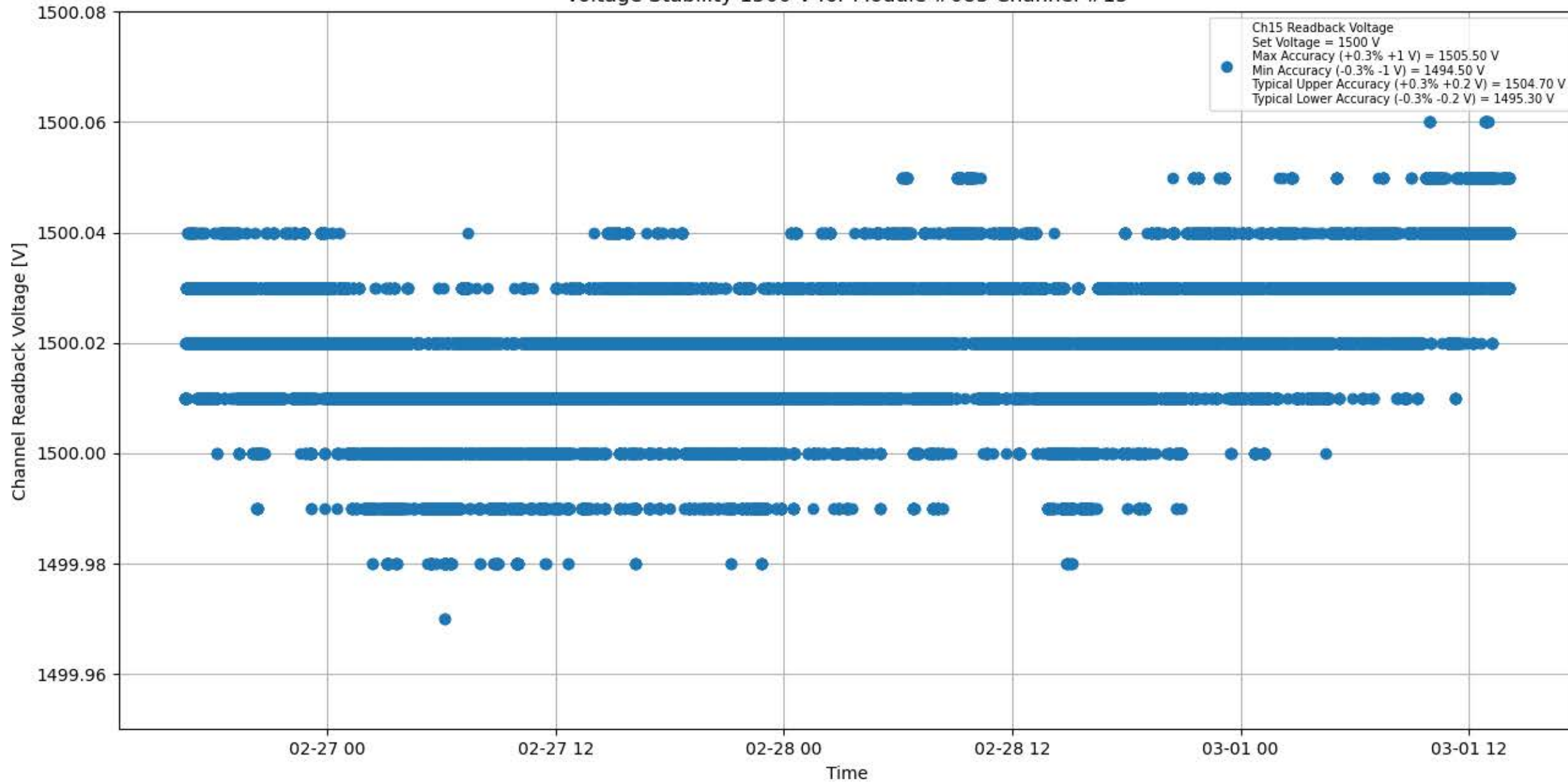
Voltage Stability 1500 V for Module #083 Channel #15
