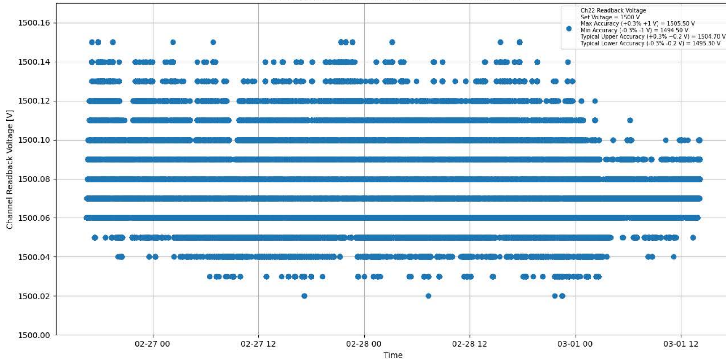
Voltage Stability 1500 V for Module #083 Channel #22
