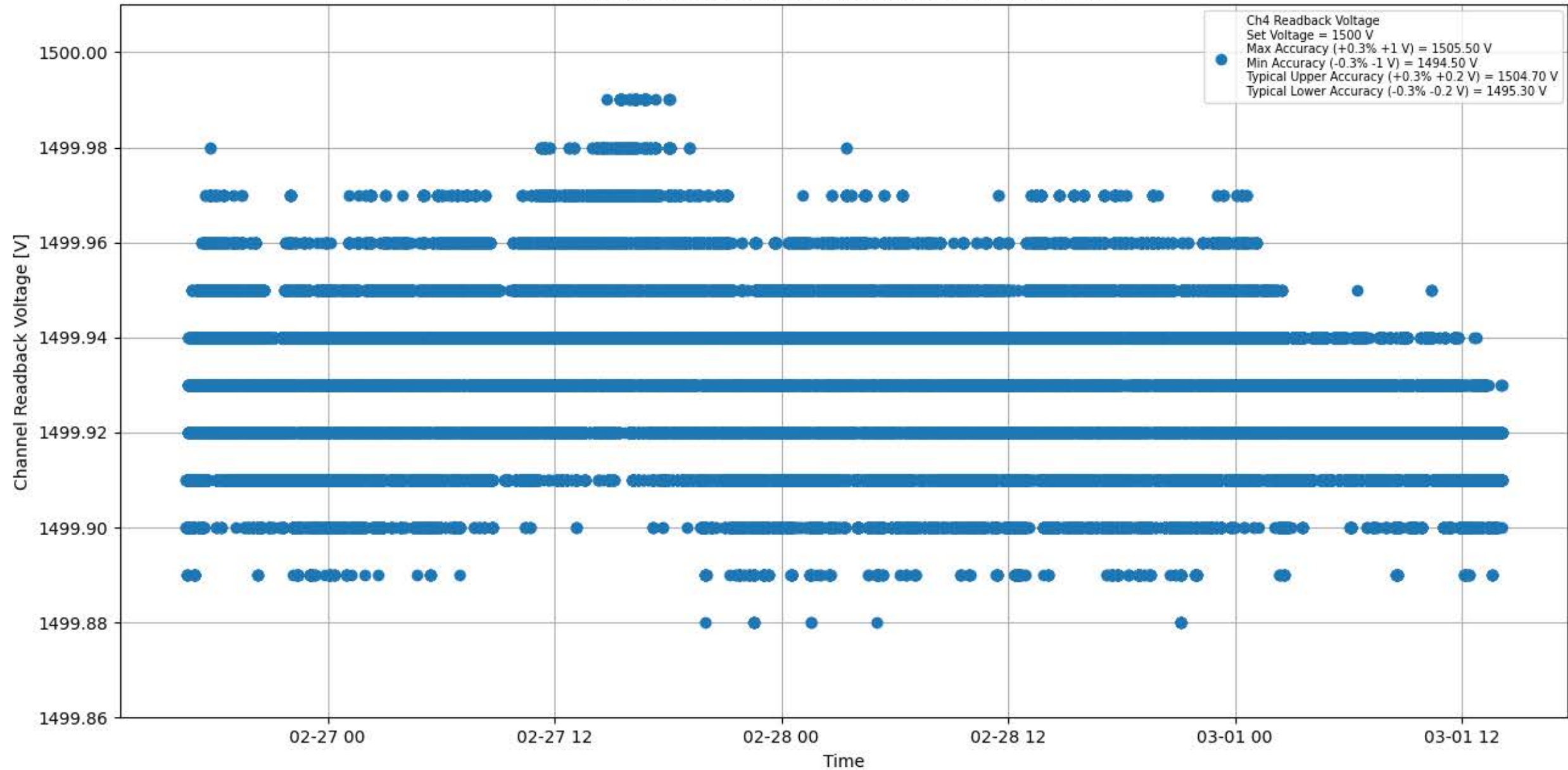
Voltage Stability 1500 V for Module #083 Channel #4
