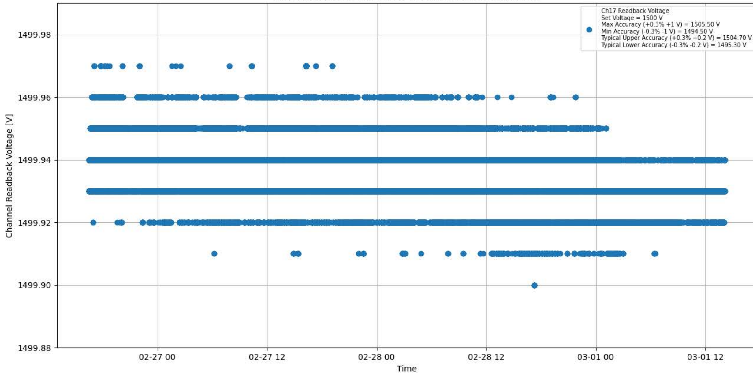
Voltage Stability 1500 V for Module #083 Channel #17
