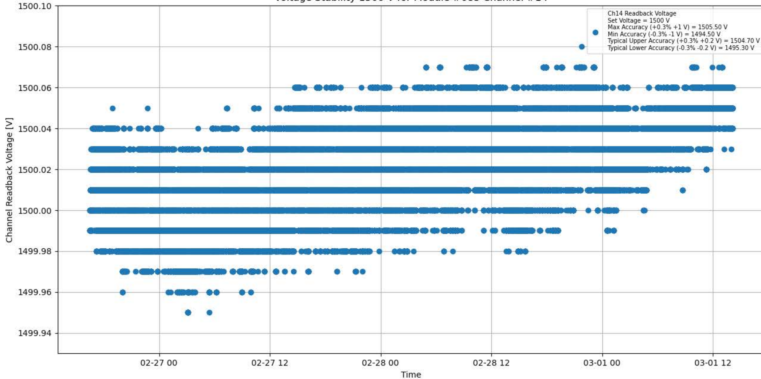
Voltage Stability 1500 V for Module #083 Channel #14
