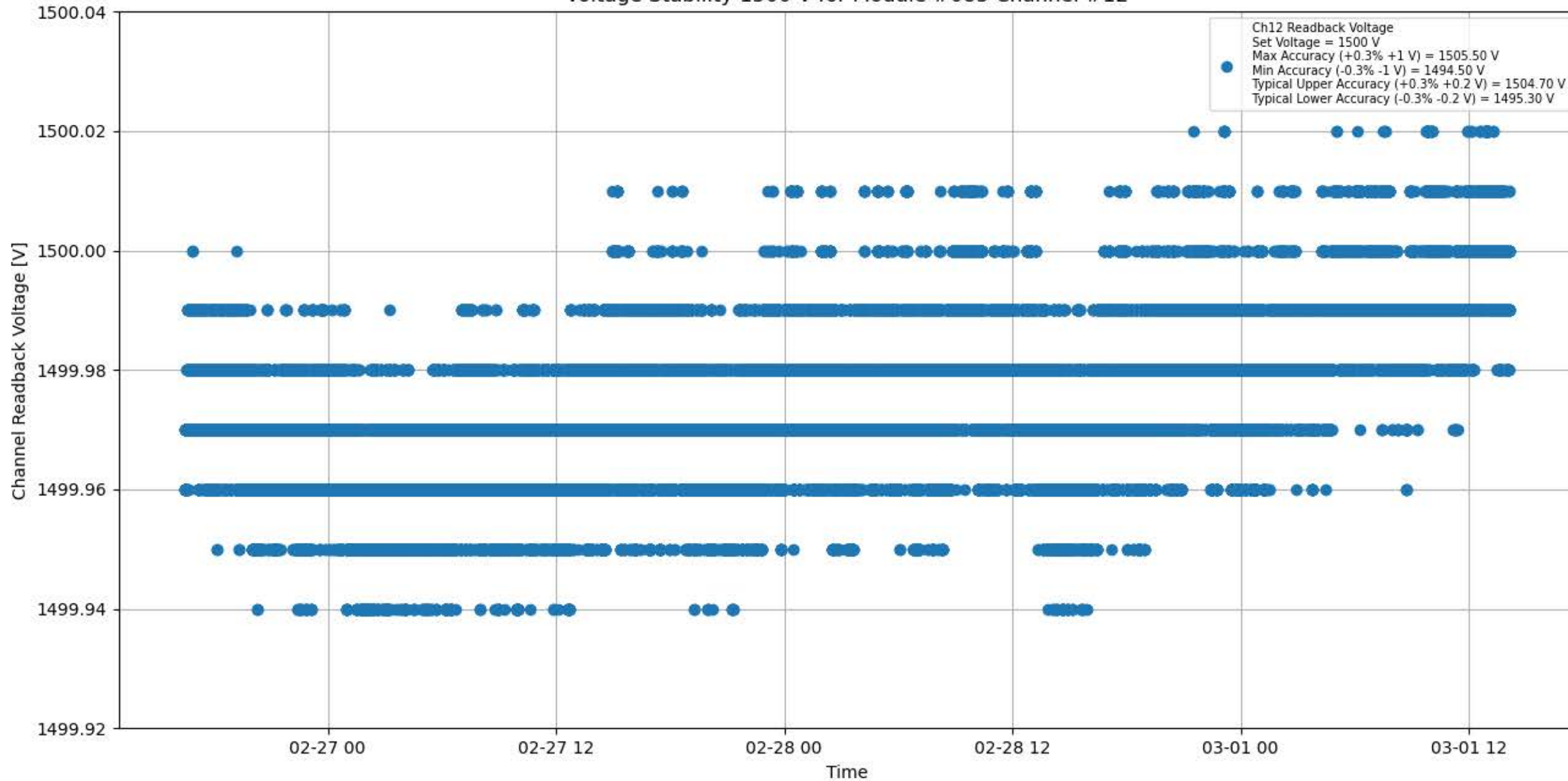
Voltage Stability 1500 V for Module #083 Channel #12
