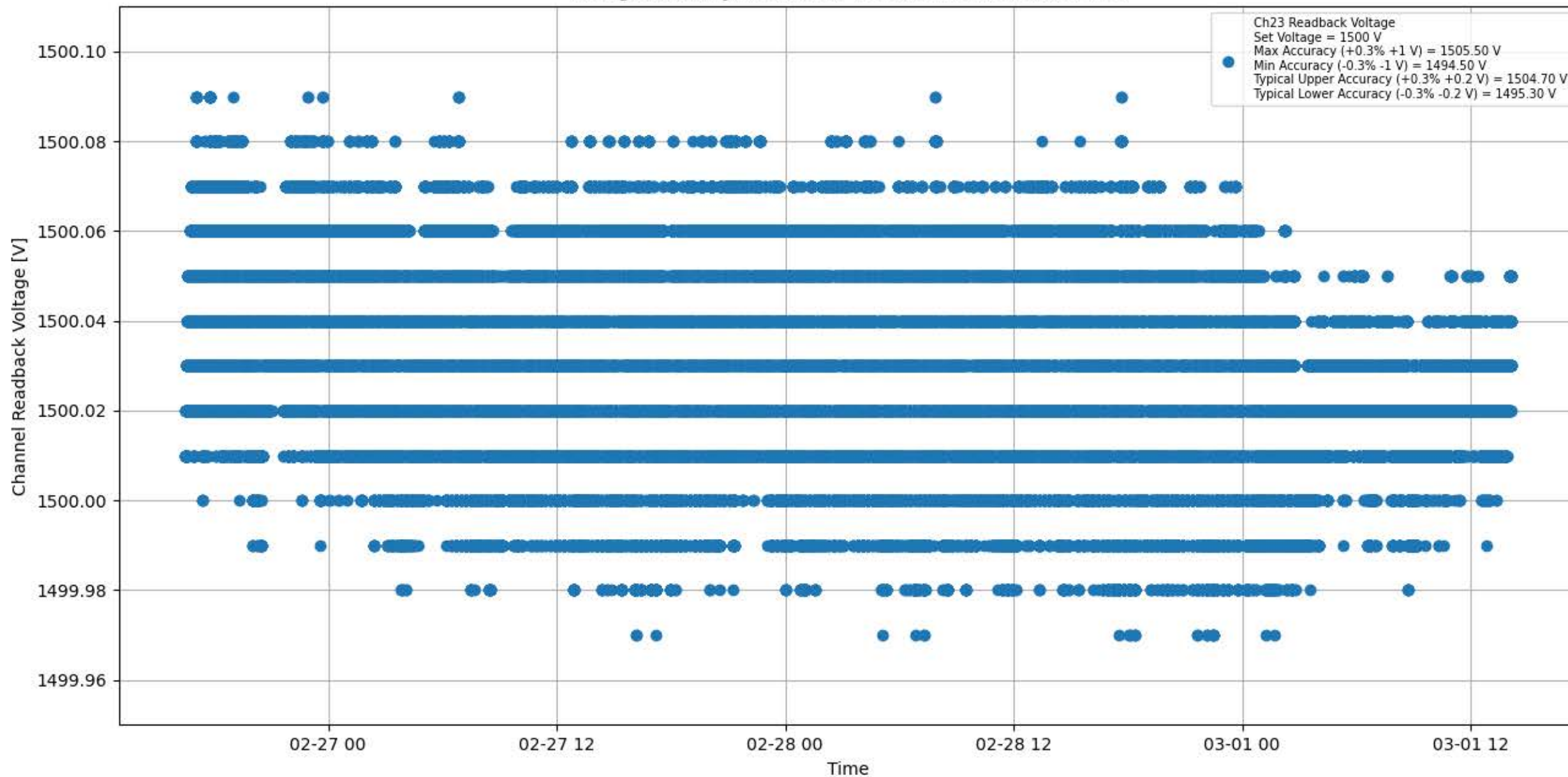
Voltage Stability 1500 V for Module #083 Channel #23
