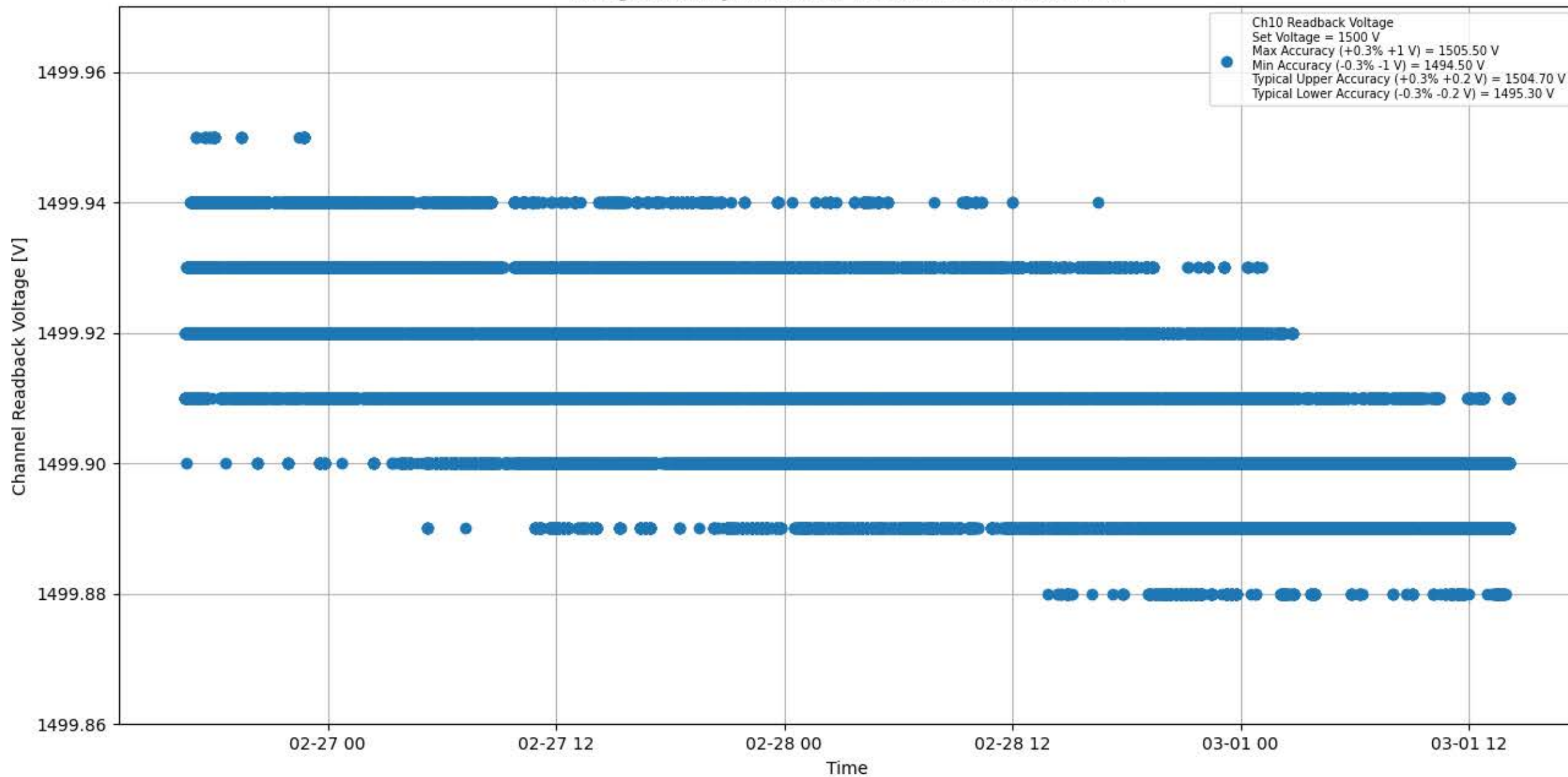
Voltage Stability 1500 V for Module #083 Channel #10
