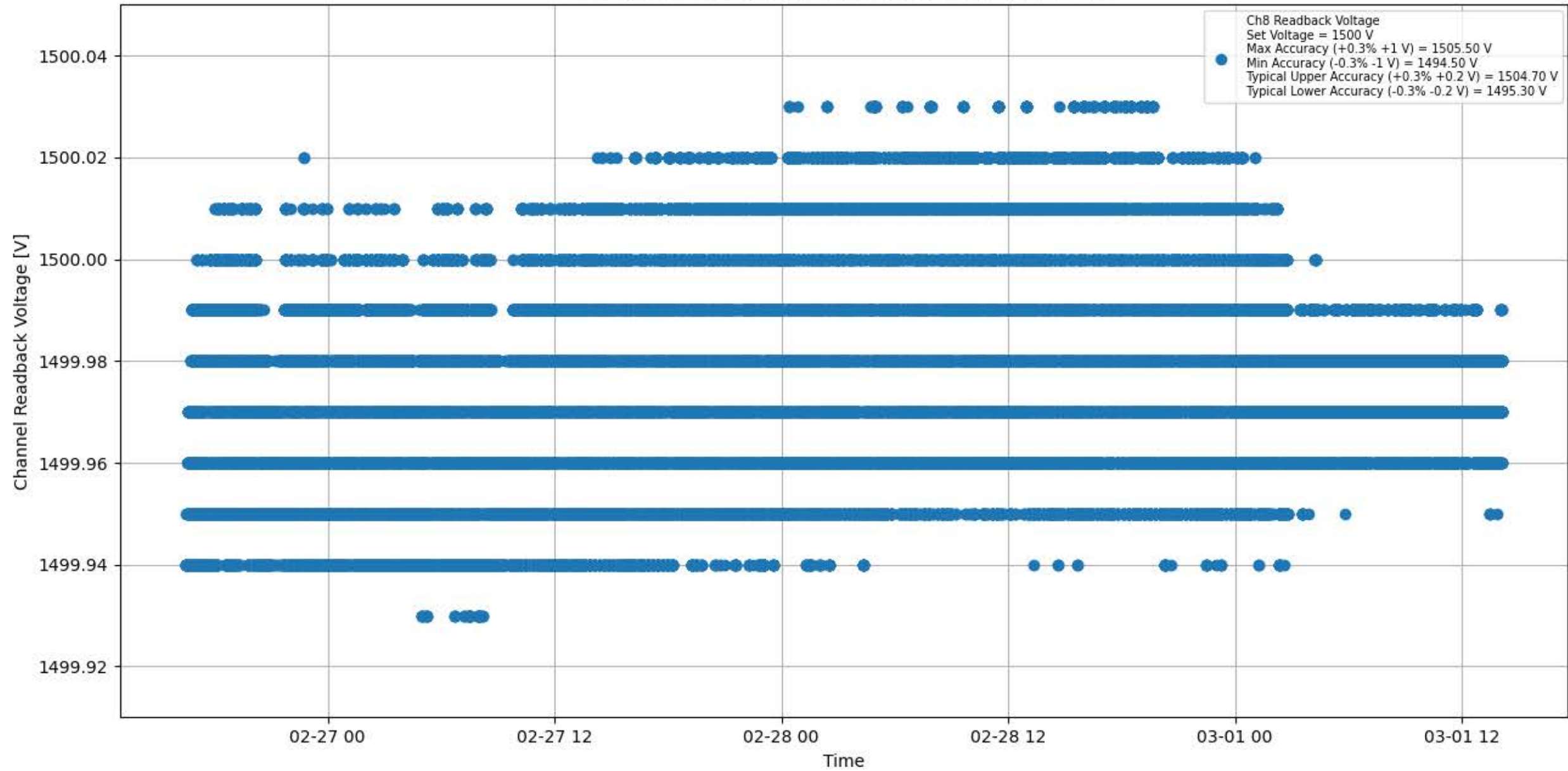
Voltage Stability 1500 V for Module #083 Channel #8
