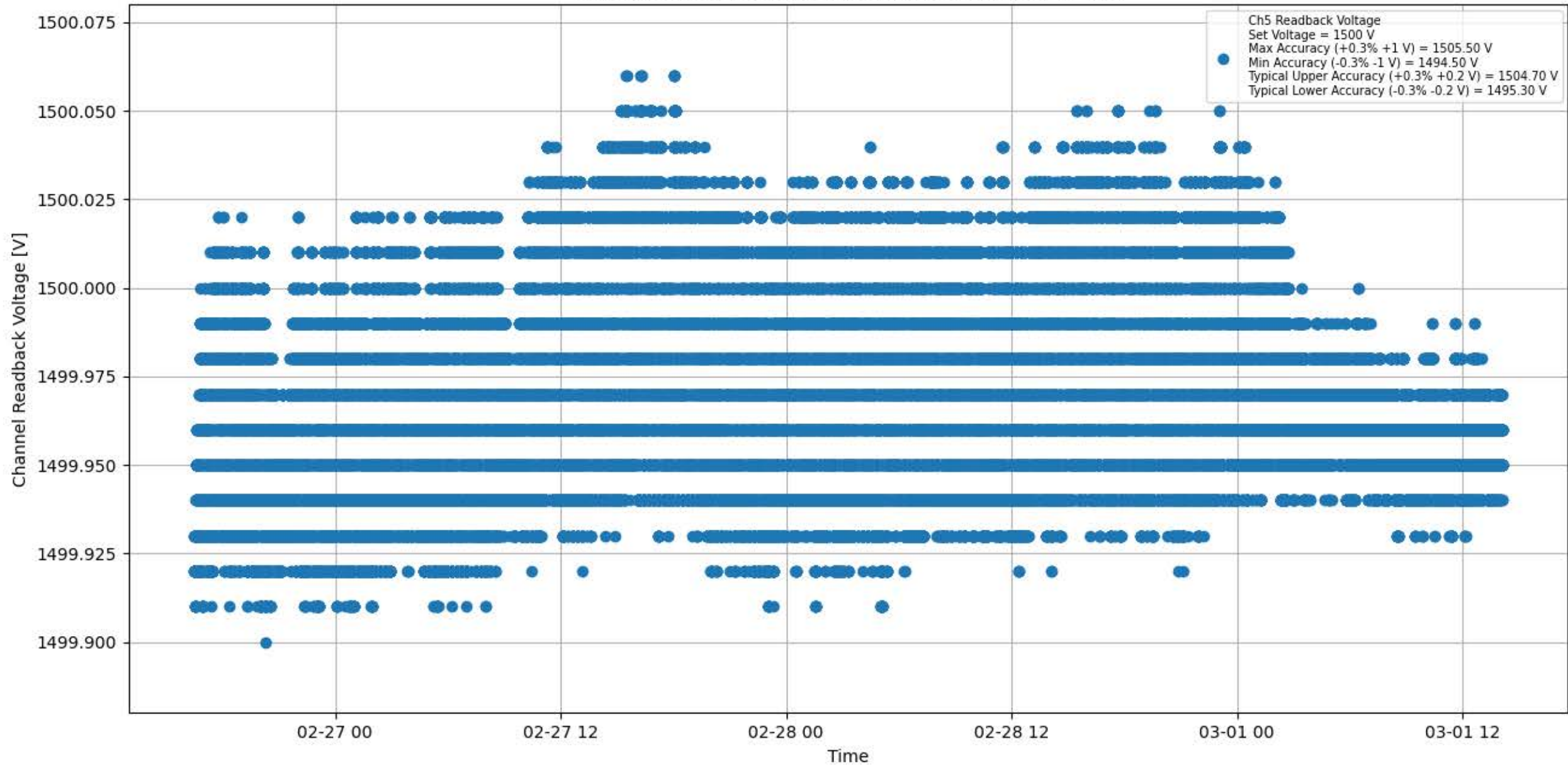
Voltage Stability 1500 V for Module #083 Channel #5
