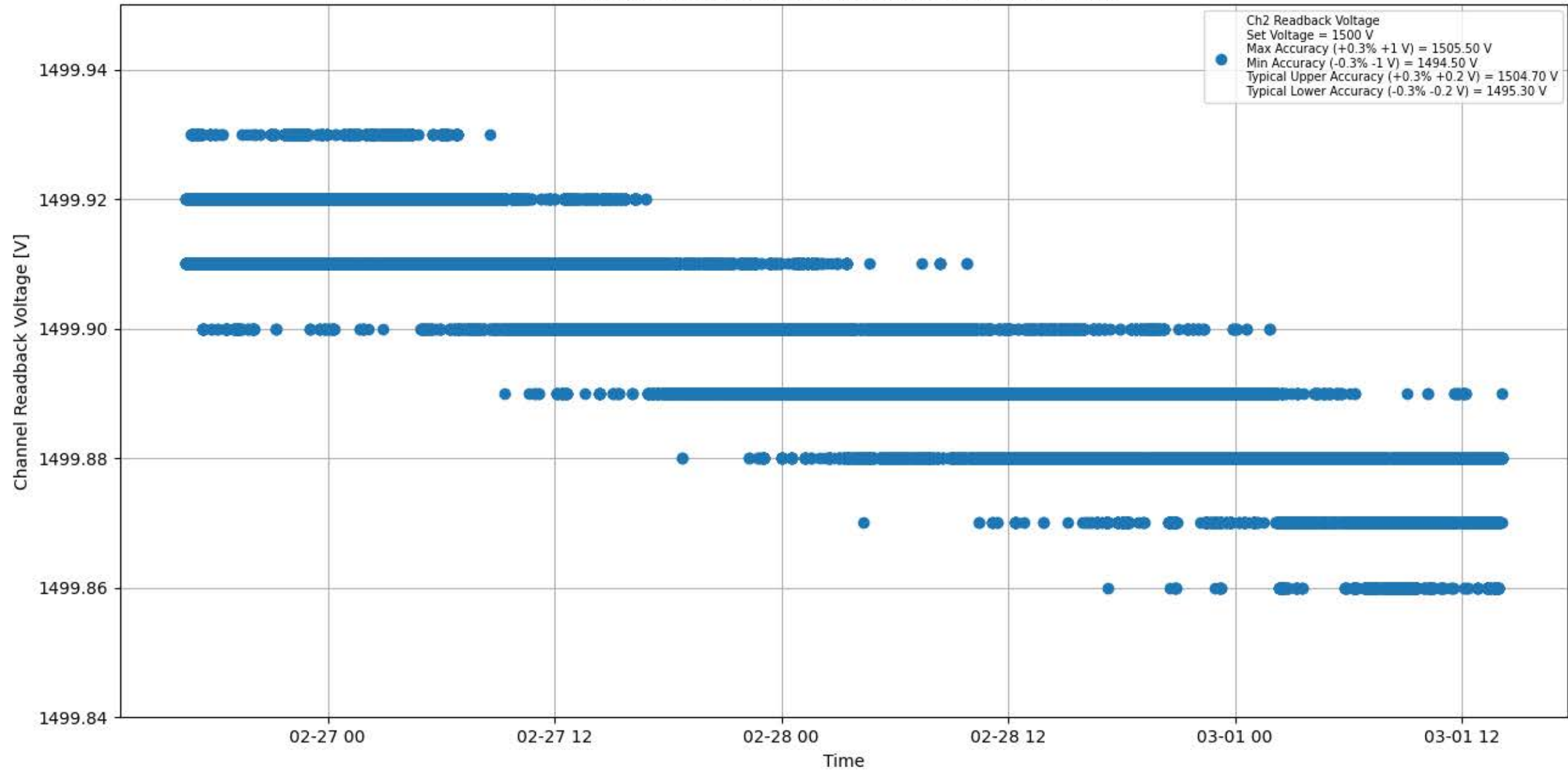
Voltage Stability 1500 V for Module #083 Channel #2
