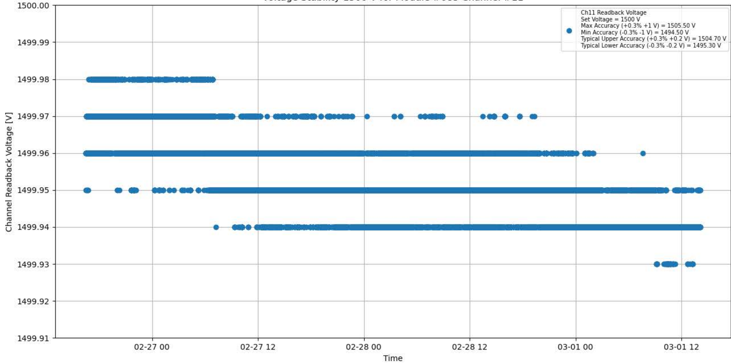
Voltage Stability 1500 V for Module #083 Channel #11
